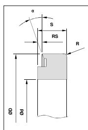
type NN without groove
