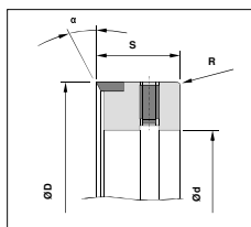
type NS-TCT with screw fixing
